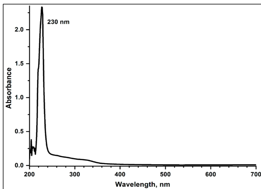
Figure 4. Absorption spectrum of [\text{CuL}_2]\text{Br}_2 at a concentration of 0.1 mM in the range of 200–700 nm, in the medium for measuring OJIP-kinetics at room temperature.
