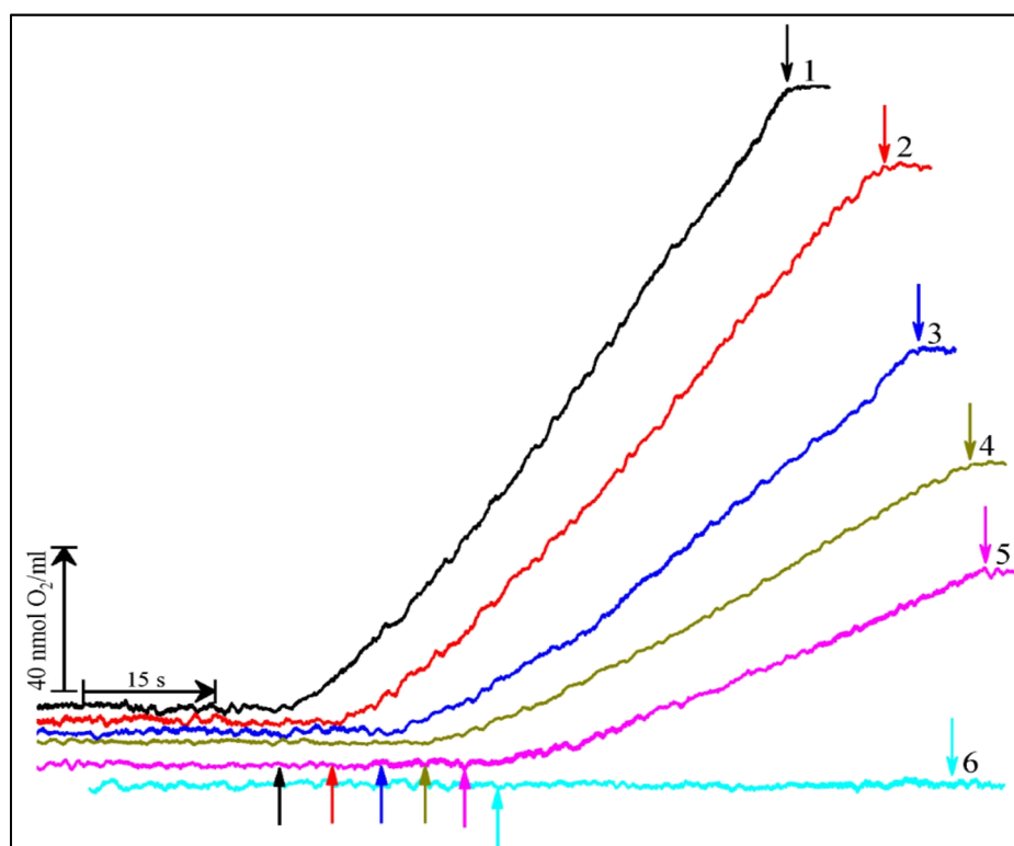
Figure 2. Kinetics of the PSII membranes oxygen evolution in the absence of any
