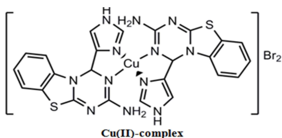
Figure 1. Cu(II)-complex (Bis{4H-1,3,5-triazino [2,1-b]benzothiazole-2-amine,4-(2-imidazole)} copper (II) bromide).
