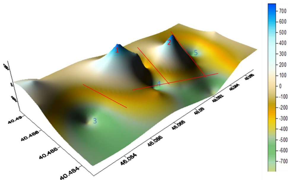
Figure 11. The model of the stress-deformation state of the geomagnetic field in the waste and landslide areas of Dashkasan skarn-iron ore group beds in 3D format
