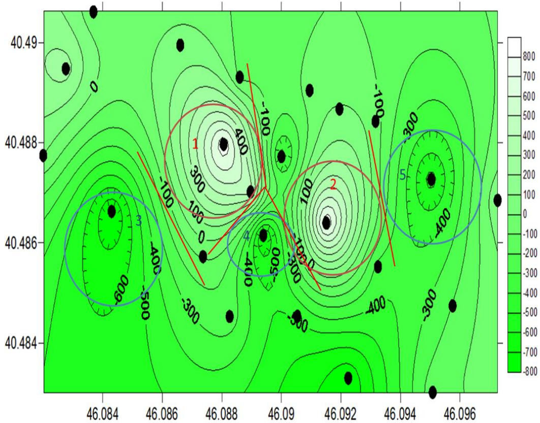
Figure 10. Map of the stress-deformation state of the geomagnetic field in the waste and landslide areas of Dashkasan skarn-iron ore group beds in 2D format
